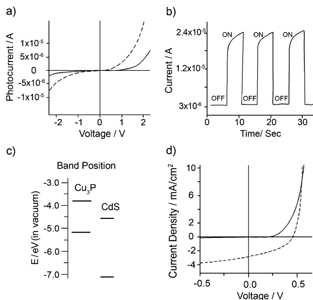
Figure 5. a) I – V characteristics of the photodetector ITO/PEDOT:PSS/Cu 3 P/Al in the dark (—) and under illumination (---; Xe lamp) using a 2 V bias and 100 mWcm −2 white-light intensity. b) Photo-current response of the photodetector using the white-light source. This has been performed up to three cycles and for all cycles it behaves the same. c) Band positions of Cu 3 P and CdS. d) I – V characteristics of a photovoltaic device with a Cu 3 P–CdS p–n junction based on Cu 3 P nanoplatelets with a layered structure of ITO/PEDOT:PSS/Cu 3 P:CdS/Al, in the dark (—) and under white-light illumination conditions (---). Open circuit voltage ( V OC ) = 0.46, short circuit current density ( I SC ) = 2.7, fill factor (FF) = 0.39, efficiency = 0.49 %.
